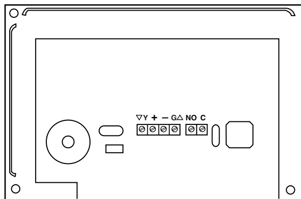
Figure 2 - FA270RF Wiring Connections
