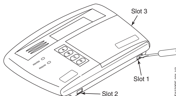
Figure 1 – Removing the FA270RF Case Back
